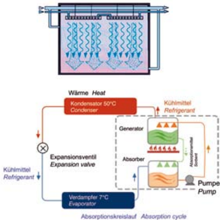
Kühldecke / ceiling with integrated cooling system
